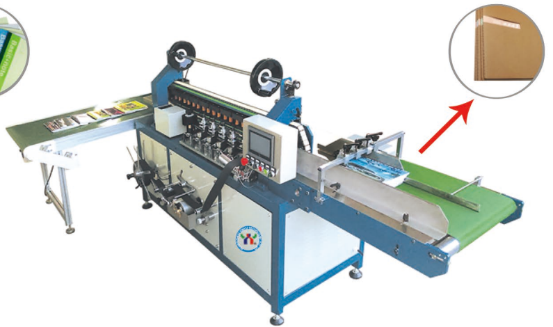
YYHB-620P PACK BACK MACHINE
